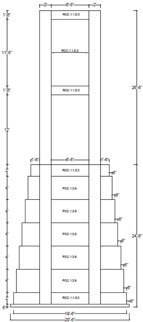
Left Abutment
