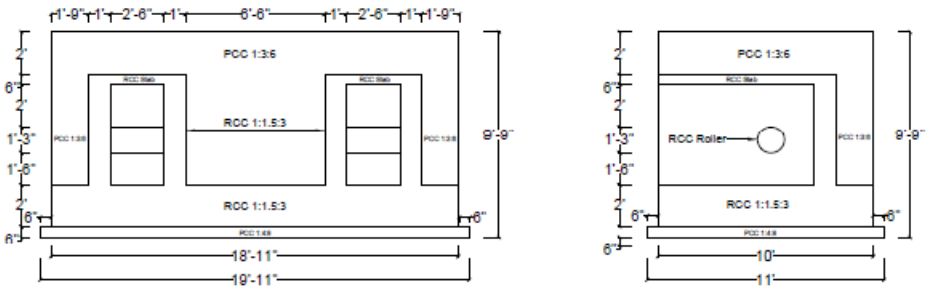
Left Abutment Main Anchor Block
