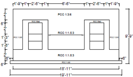
Left Abutment Main Anchore Block
