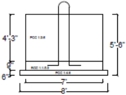
Wind Anchore Block
