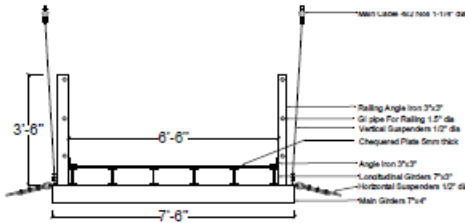
Deck Slab
