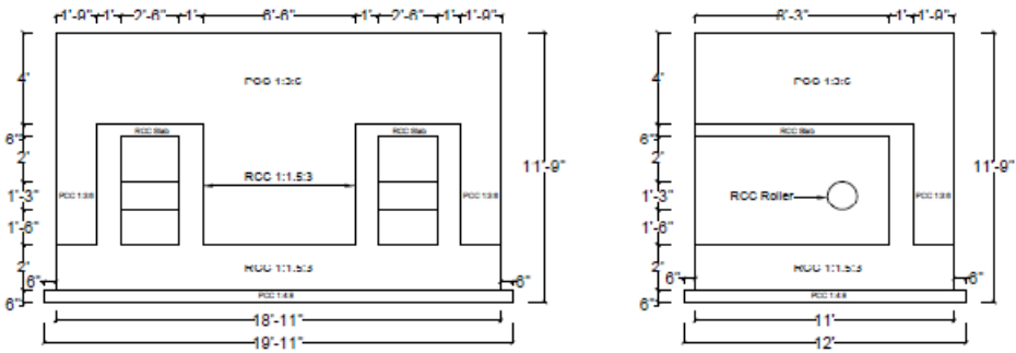
Right Abutment Main Anchor Block
