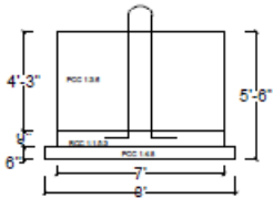
Wind Anchor Block
