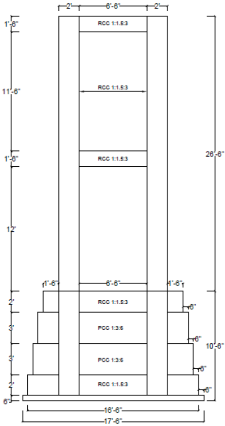
Right Abutment
